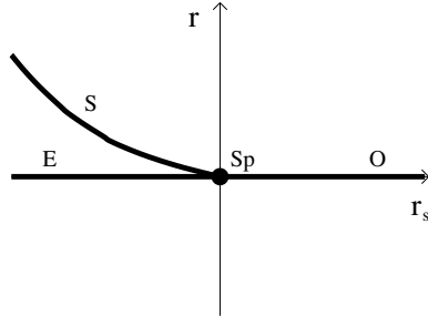
Figure 10. Schematic mean-field phase diagram for boundary DP. The transitions are labelled by O = ordinary, E = extraordinary, S = surface, and Sp = special.
